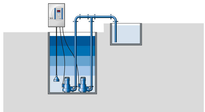
Pneumatic measurement/bubbler system with pressure bell
