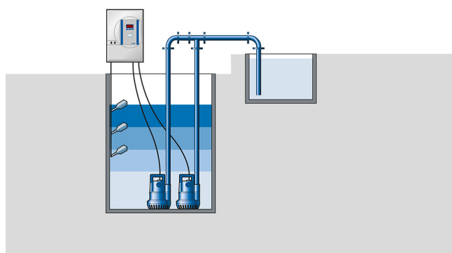
Level detection via float switches
